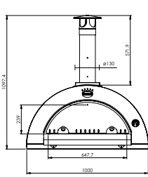
FAMILY 80x60 cm - kg 112
