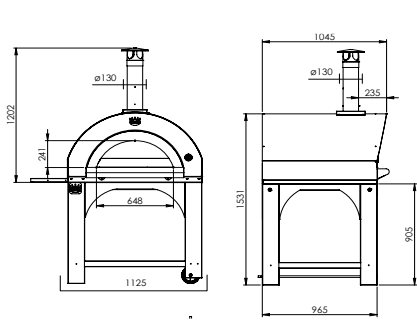
PULCINELLA 100x80 cm - kg 275
