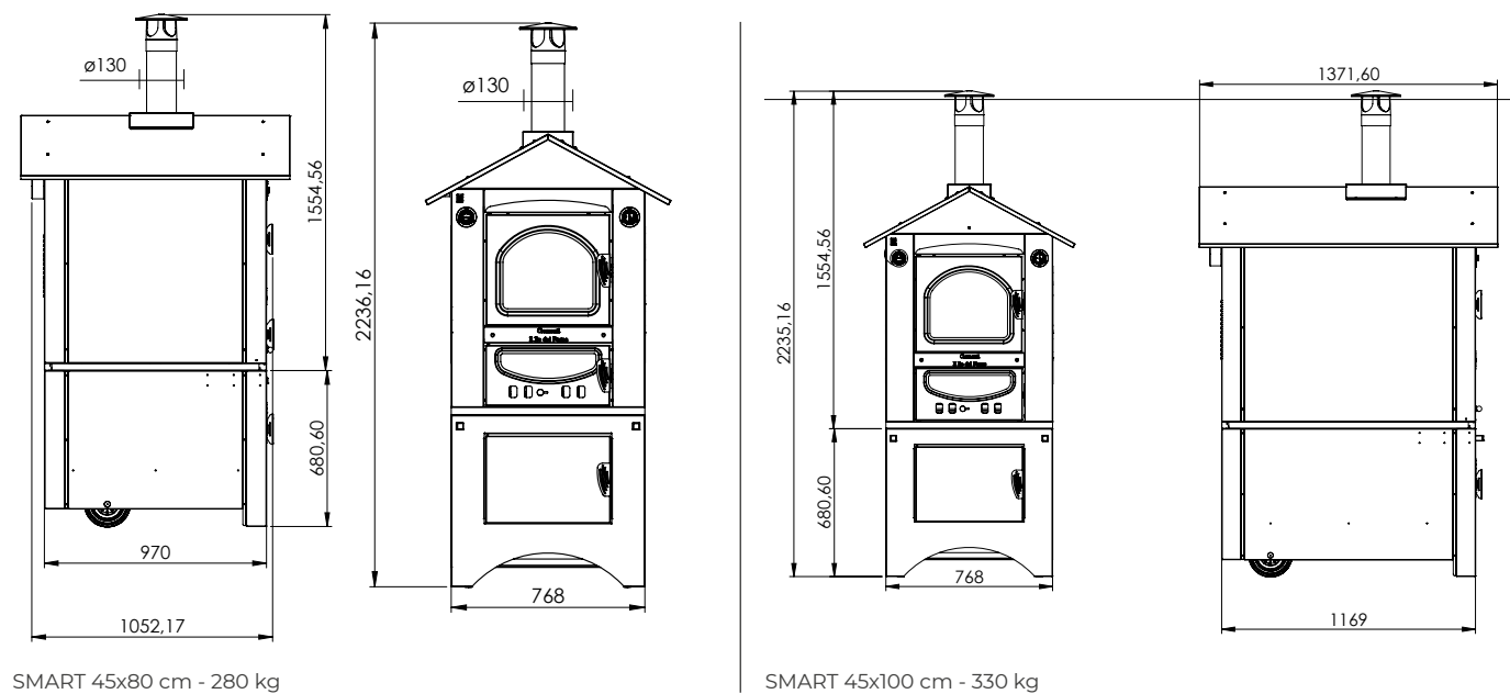
SMART 45x80 cm - 280 kg
