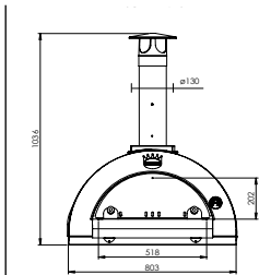
FAMILY 60x60 cm - kg 95
