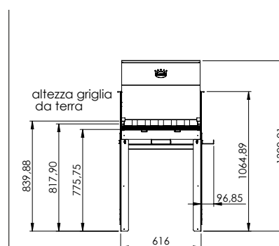
SUPER FLIPPER - 55 kg
