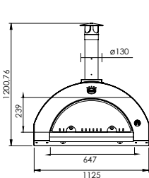
FAMILY 100x80 cm - kg 230
