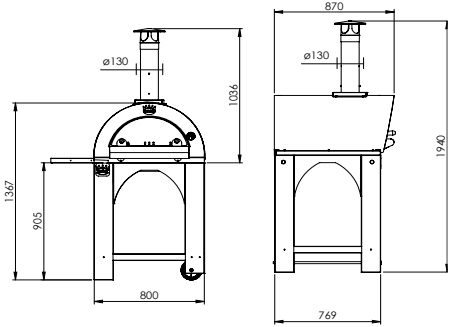
PULCINELLA 60x60 cm - Kg 130
